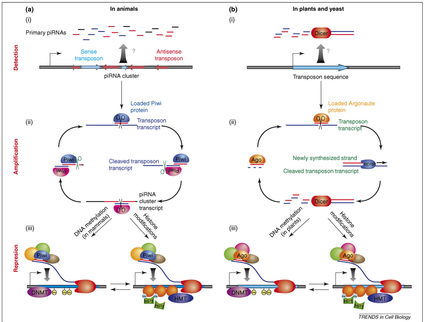
Figure 1. Eukaryotic small RNA-based transposon silencing relies on three linked steps: detection, amplification and repression. (a) (i) In animals, 24–30-nucleotide primary piRNAs are processed from long RNA precursors transcribed from defined loci called piRNA clusters. Any transposon inserted in the reverse orientation in the piRNA cluster can give rise to antisense piRNAs (in red). (ii) Antisense piRNAs are incorporated into a Piwi protein (in flies, this is mostly Aubergine or Piwi) and direct its Slicer activity on sense transposon transcripts. The 3' cleavage product is bound by another Piwi protein (Ago3 in flies) and trimmed to piRNA size. This sense piRNA is in turn used to cleave piRNA cluster transcripts and to generate more antisense piRNAs. (iii) Eventually, antisense piRNAs can target the Piwi complexes to cDNA for DNA methylation and/or histone modification. (b) (i) In plants and S. pombe , transposon expression leads to dsRNA formation, through a process that is still largely unexplained. One possible source of dsRNA is the read-through transcription of inverted repeats. Another is the synthesis of the reverse strand from transposon RNA templates by an RDRP. This dsRNA is then processed into 21–24-nucleotide small RNAs by a Dicer protein. (ii) Transposon-derived siRNAs can then bind an Argonaute protein and direct cleavage of transposon transcripts. These cleaved RNAs are potential templates for RDRP-mediated reverse strand synthesis and processing of more siRNAs by Dicer. (iii) As in animals, siRNA-Argonaute complexes can target DNA and histone-modifying complexes to cDNA sequences.
