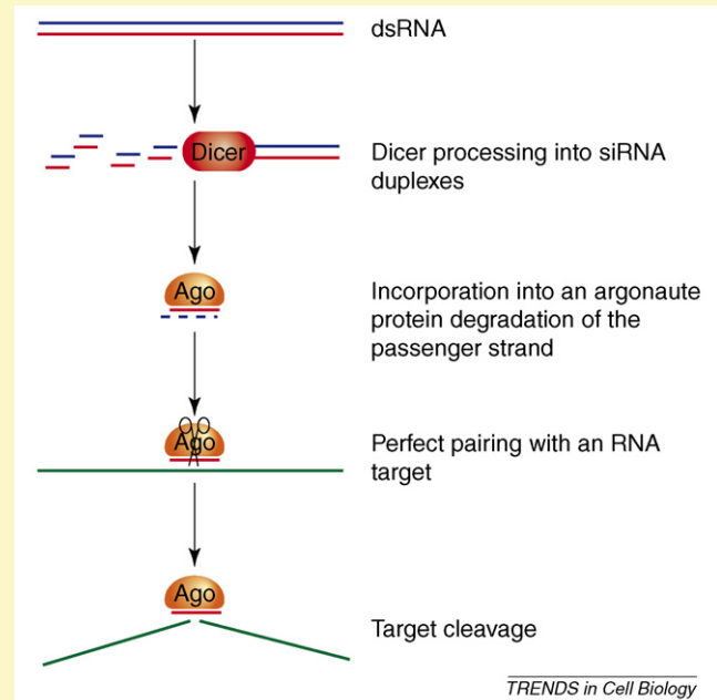
Figure 1. The siRNA pathway.
