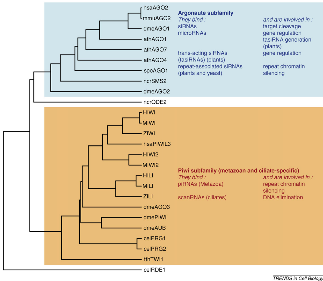
Figure 1. The Argonaute protein family. Abbreviations: ath, Arabidopsis thaliana ; cel, Caenorhabditis elegans ; dme, Drosophila melanogaster ; hsa, Homo sapiens ; mmu, Mus musculus ; ncr, Neurospora crassa ; spo, Schizosaccharomyces pombe ; tth, Tetrahymena thermophila .
