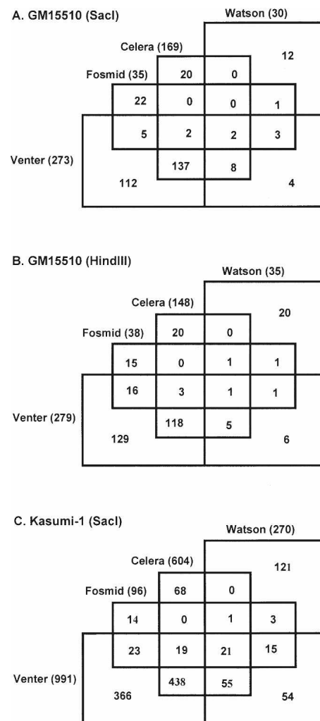
Figure 4. Genome variations in four individual genomes detected by ditags. The GM15510 ditags not mapped to HG18 were mapped against the reference ditags from the four human genome sequences of GM15510 fosmid sequences, Celera genome sequences, Venter genome sequences, and Watson genome sequences.
