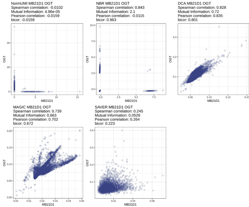
Figure 3. Spurious gene-gene correlation caused by data oversmoothing
