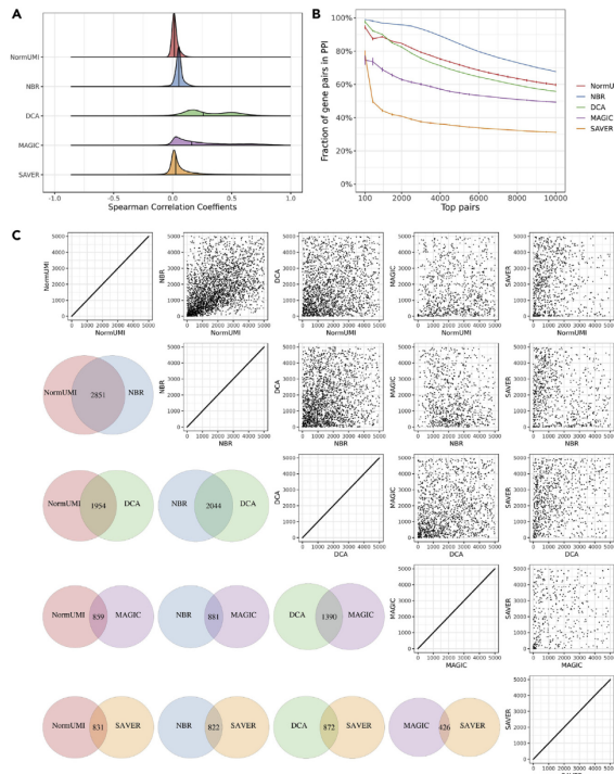
Figure 4. Noise regularization reduces spurious correlations
