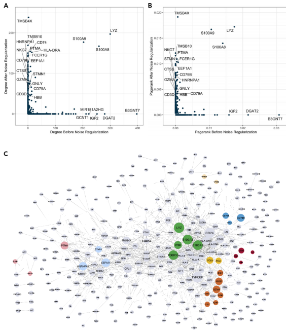
Figure 5. Gene-gene correlation network inferred from scRNA-seq data
