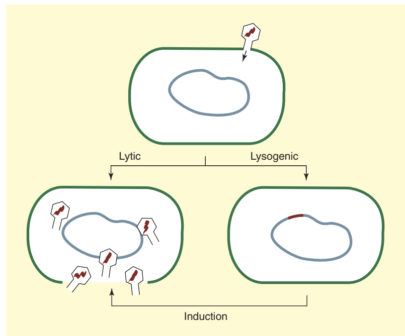
Figure 1. The life cycle of \lambda .
