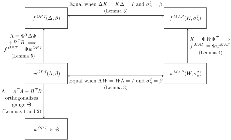
Fig. 1 An illustration of the equivalences established. Let A and B be matrices such that \text{nullspace}(A) = G and \text{nullspace}(B) = \Theta
