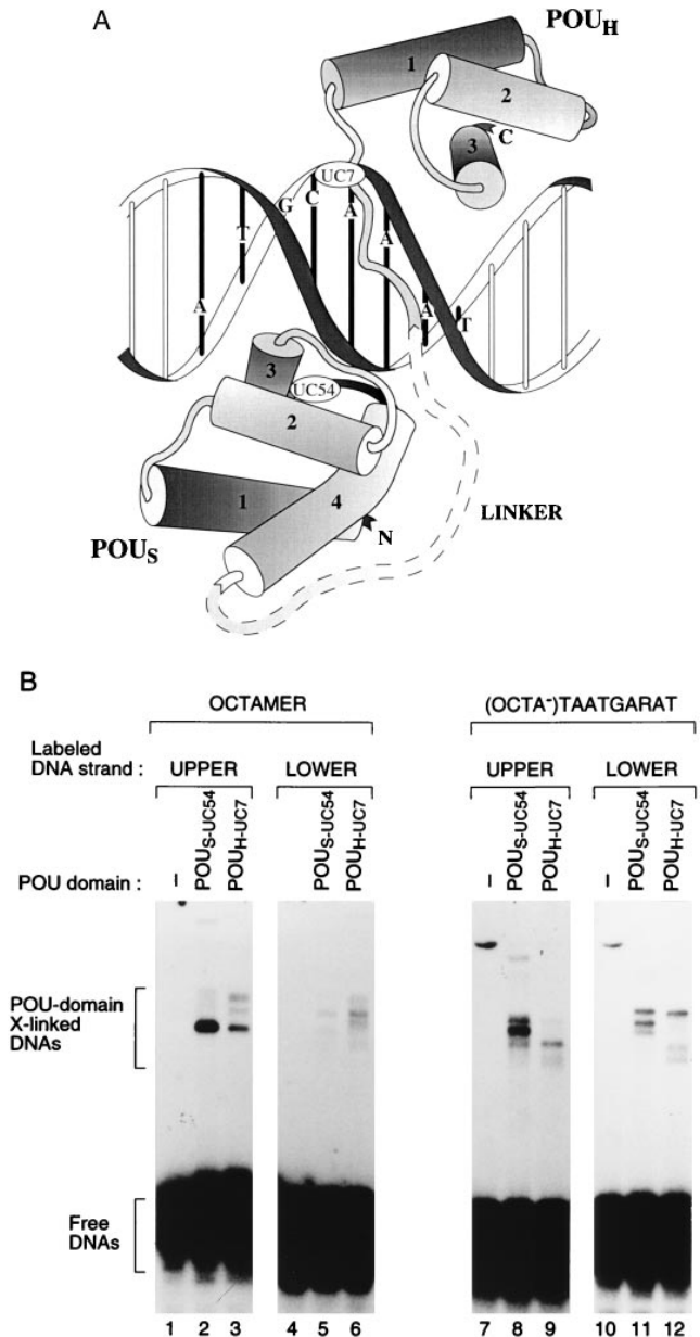
FIG. 1. Unique cysteines in the POU S and POU H domains effective for protein-DNA crosslinking. (A) Representation (adapted from refs. 2 and 4) of the Oct-1 POU domain-octamer site crystal structure with the positions of the unique cysteines used for crosslinking analysis indicated (UC54 in the POU S domain and UC7 in the POU H domain; the precise location of UC54 is hidden behind helix 2 on the turn between helices 3 and 4). (B) SDS/PAGE analysis of crosslinked protein-DNA complexes after UV irradiation of POU domain-binding reactions containing no protein (lanes 1, 4, 7, and 10), POU S -UC54 protein (lanes 2, 5, 8, and 11), or POU H -UC7 protein (lanes 3, 6, 9, and 12). Shown are crosslinked complexes formed on the upper and lower strands of the histone H2B octamer and the (OCTA - )TAATGARAT sites, as indicated.
