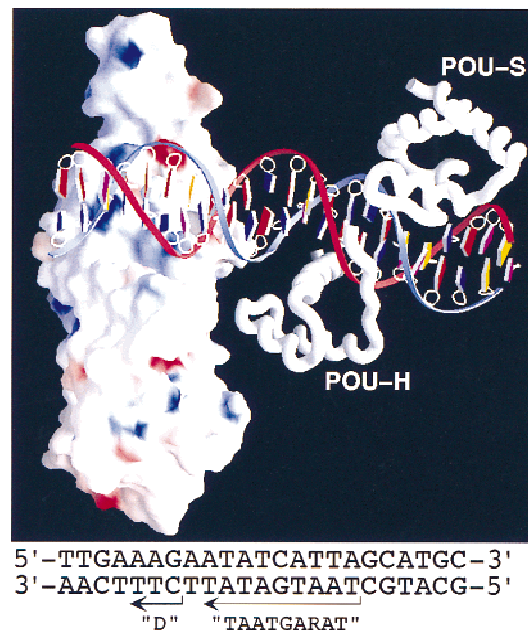
Figure 8. Model of VP16 bound to a TAATGARAT element with the Oct-1 POU domain. The presentation of VP16 is similar to that shown in Fig. 7B. The nucleotide sequence of the DNA in the model is shown at the bottom and originates from the HSV ICP0 gene promoter. In the graphic, the bases are color coded as follows: A (red), T (blue), G (yellow), and C (purple). The blue DNA strand represents the top strand; the red strand represents the bottom strand of the sequence shown below. The Oct-1 POU S (POU-S) and POU H (POU-H) domain structures and the Oct-1 DNA-binding site structure are from Klemm et al. (1994).
