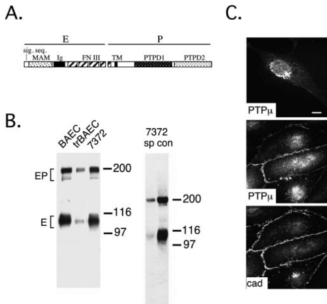
FIG. 1. Endogenous PTP \mu expression in bovine endothelial cells. A, the domain structure of PTP \mu is outlined with the signal sequence (sig. seq.) and the MAM, immunoglobulin (Ig), fibronectin type III repeat (FN III), transmembrane (TM), and tandem catalytic (PTPD1/D2) domains indicated above the diagram. The positions of the E- and P-subunits (amino acids 23–638 and 639–1452, respectively) are indicated. B, lysates from confluent cultures of BAEC, trBAEC, and GM7372 cells (7372) (left panel) and sparse (sp; ~40% confluent) and confluent (con) GM7372 cells (right panel) were analyzed by immunoblotting with anti-PTP \mu antibody BK2. 40 \mu g of protein were loaded for each lysate. Brackets indicate the positions of the non-proteolytically processed protein (EP) and the proteolytically processed E-subunit (E). Pulse-chase labeling studies suggested that the lower band(s) for the EP protein represents the initial protein product prior to glycosylation and subsequent processing. The migration positions of relative molecular mass markers (in kilodaltons) are shown to the right of each panel. C, subconfluent GM7372 cells were fixed and stained with anti-PTP \mu antibody SK7 (upper panel), and confluent cells were stained sequentially with antibody SK7 (middle panel) and anti-VE-cadherin antibody 45C6 (cad; lower panel) as described under “Experimental Procedures.” Scale bar = 10 \mu m.
