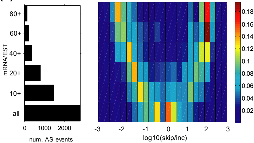
Figure S2. Distribution of frame-preserving cassette exons in terms of relative isoform abundance. (a) Human and (b) mouse data are shown. Refer to the legend of Figure 1 in the main text for details. The bimodal distribution (when a threshold of supporting transcripts was applied) is very similar to that observed for all cassette exons. This suggests that as the transcriptome is sampled more deeply, it is easier to find low-abundance splicing isoforms. This low abundance is largely independent of NMD. Also note that, in both Figure 1 and Figure S2, the peak of cassette exons with rare-skipping is almost twice that of cassette exons with rare-inclusion, which implies that leaky or aberrant exon skipping is more prevalent than inclusion. As an alternative interpretation, it is easier for random mutations to attenuate splicing signals than to create them in intronic sequences. These observations cannot be explained by NMD either.
