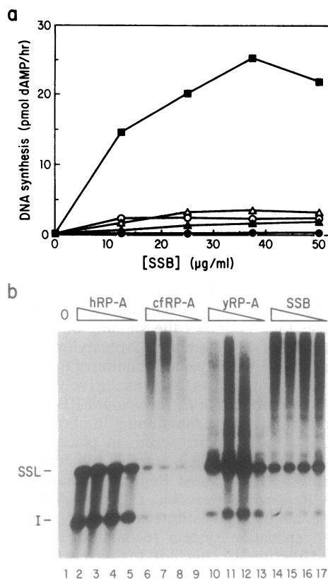
FIG. 4. C. fasciculata RP-A substitution in SV40 replication reactions. (a) Human RP-A (■), yeast RP-A (Δ), C. fasciculata RP-A (▲), E. coli SSB (○), and T4 gene 32 protein (●) at 0–50 \mu\text{g/ml} were incubated with optimized amounts of T-Ag, topoisomerase I, topoisomerase II, proliferating-cell nuclear antigen, replication factor C, fraction IIA (which contains DNA polymerases \alpha and \delta and maturation factors), and SV40 origin-containing plasmid, and DNA synthesis was measured. (b) Samples of the replication products were analyzed on denaturing agarose gels. Reactions contained the following concentrations of the indicated proteins. Lanes: 1, 0 \mu\text{g/ml} ; lanes 2, 6, 10, and 14, 50 \mu\text{g/ml} ; lanes 3, 7, 11, and 15, 37.5 \mu\text{g/ml} ; lanes 4, 8, 12, and 16, 25 \mu\text{g/ml} ; lanes 5, 9, 13, and 17, 12.5 \mu\text{g/ml} . For human RP-A (lanes 2–5), 10-fold less of the replication products was analyzed than in all other lanes. The positions of unit-length single-stranded linear molecules (SSL) and denatured form I molecules (I) are indicated. hRP-A, human RP-A; cfRP-A, C. fasciculata RP-A; yRP-A, yeast RP-A.
