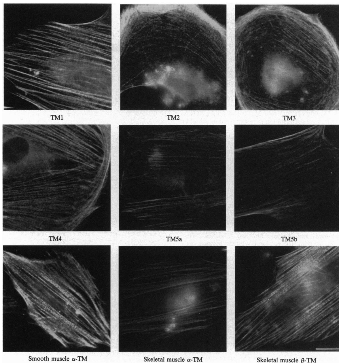
FIG. 3. Immunofluorescence showing that all HA-tagged isoforms localize and integrate into the actin-containing stress fibers of REF 52 cells. (Bar = 20 \mu m.)
