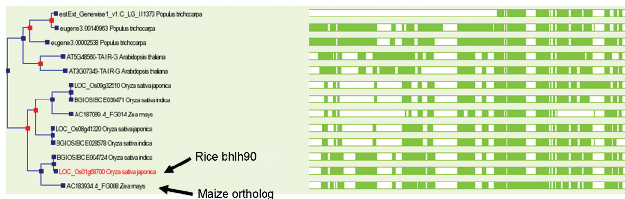
Figure 3. The rice bhlh90 gene tree (partial) showing the orthologous genes between rice, maize, A. thaliana and poplar. The full tree can be viewed at http://tinyurl.com/3clrjv . Note the bhlh90 gene is mapped in the region shown in Figure 2, but its maize gene ortholog is a predicted gene and has not been studied functionally. The solid box on the right shows the aligned regions in the proteins. It is expected that there are more maize orthologs to be identified after the maize genome sequence becomes complete.
